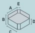
MODUL CORNER SEAT / A 75 cm / B 58 cm / C 75 cm / D 33 cm / E 22 cm
